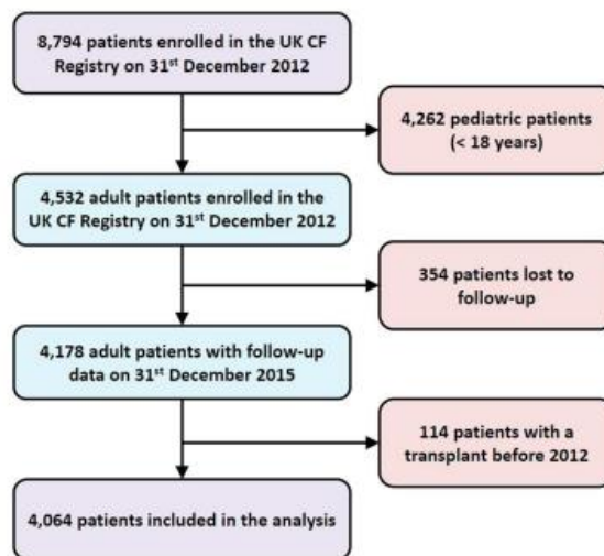
Figure: 1. Process for choosing patients and assembling data.
